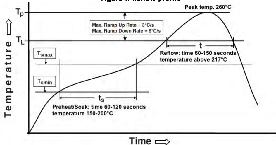
Figure 1: Reflow profile
